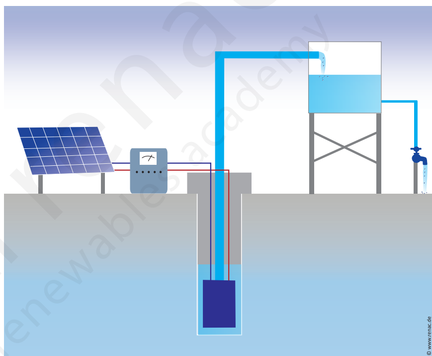
Figure 1: Solar pumping system 8
